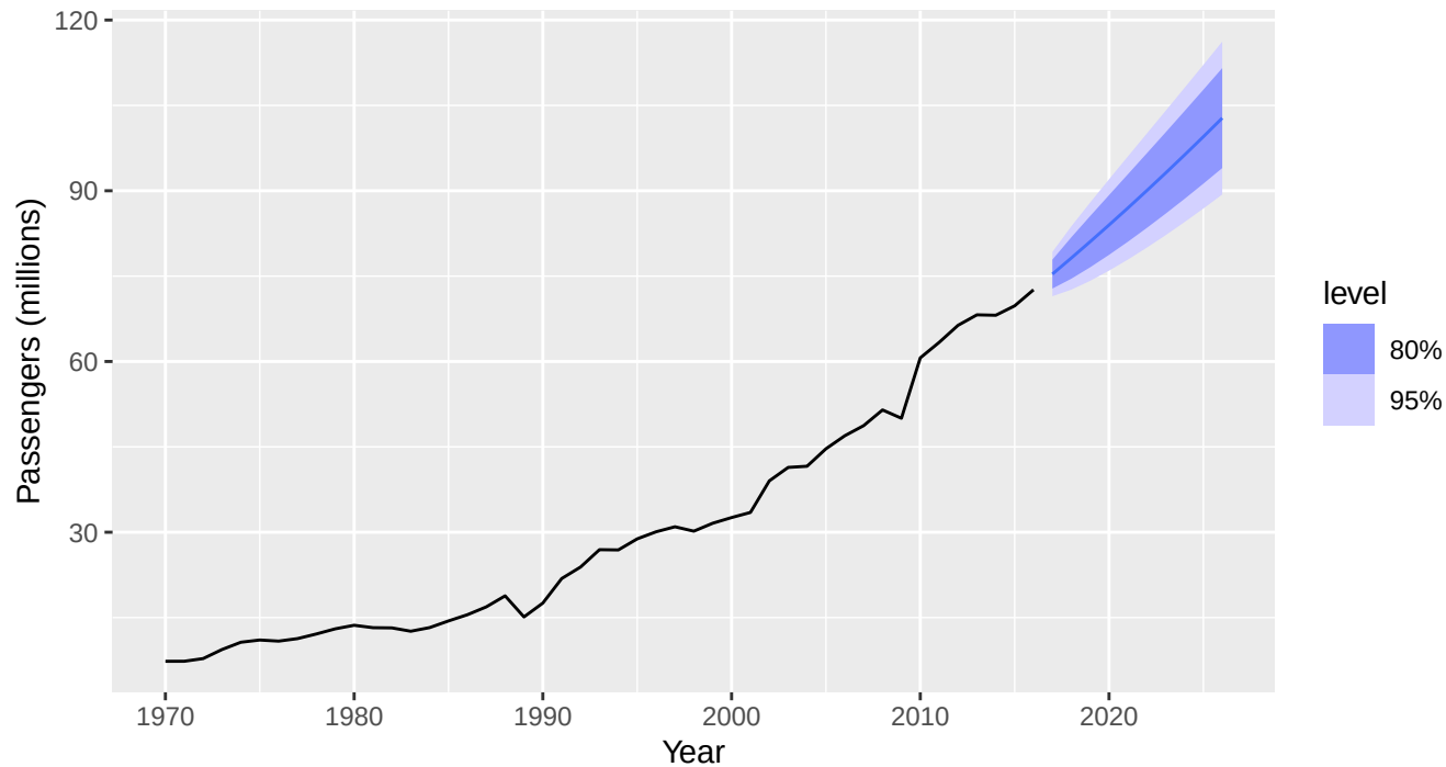
ARIMA(0,2,1) with constant
