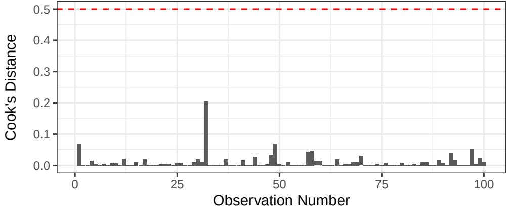
Cook's Distance
