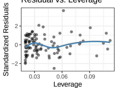
Residual vs. Leverage
