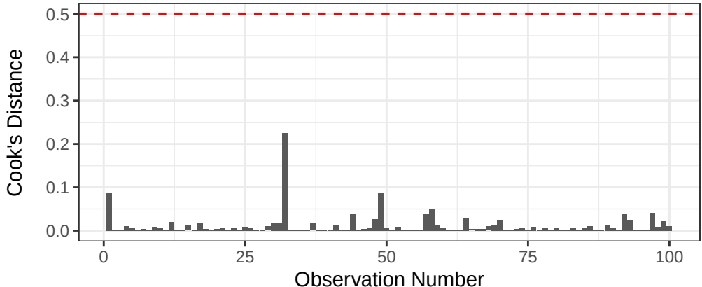
Cook's Distance
