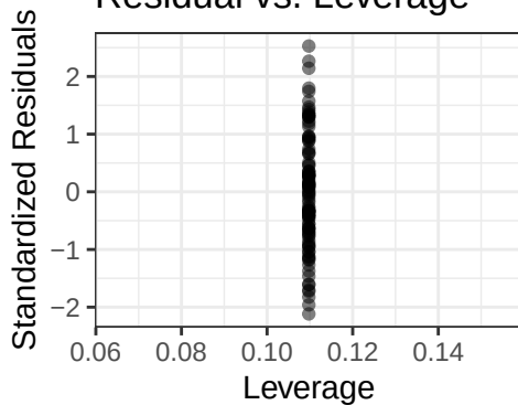
Residual vs. Leverage
