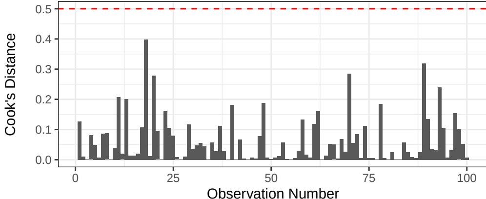
Cook's Distance
