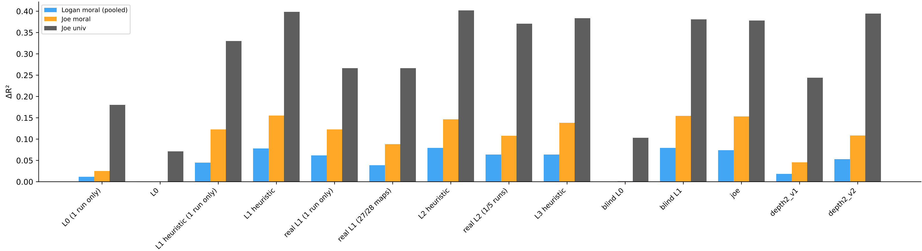
\Delta R^2 by model \times experiment
