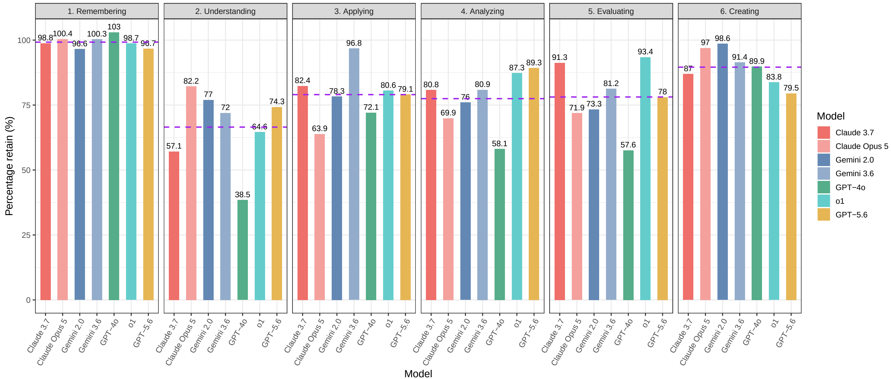
Model Accuracy Comparison: Report vs Baseline
