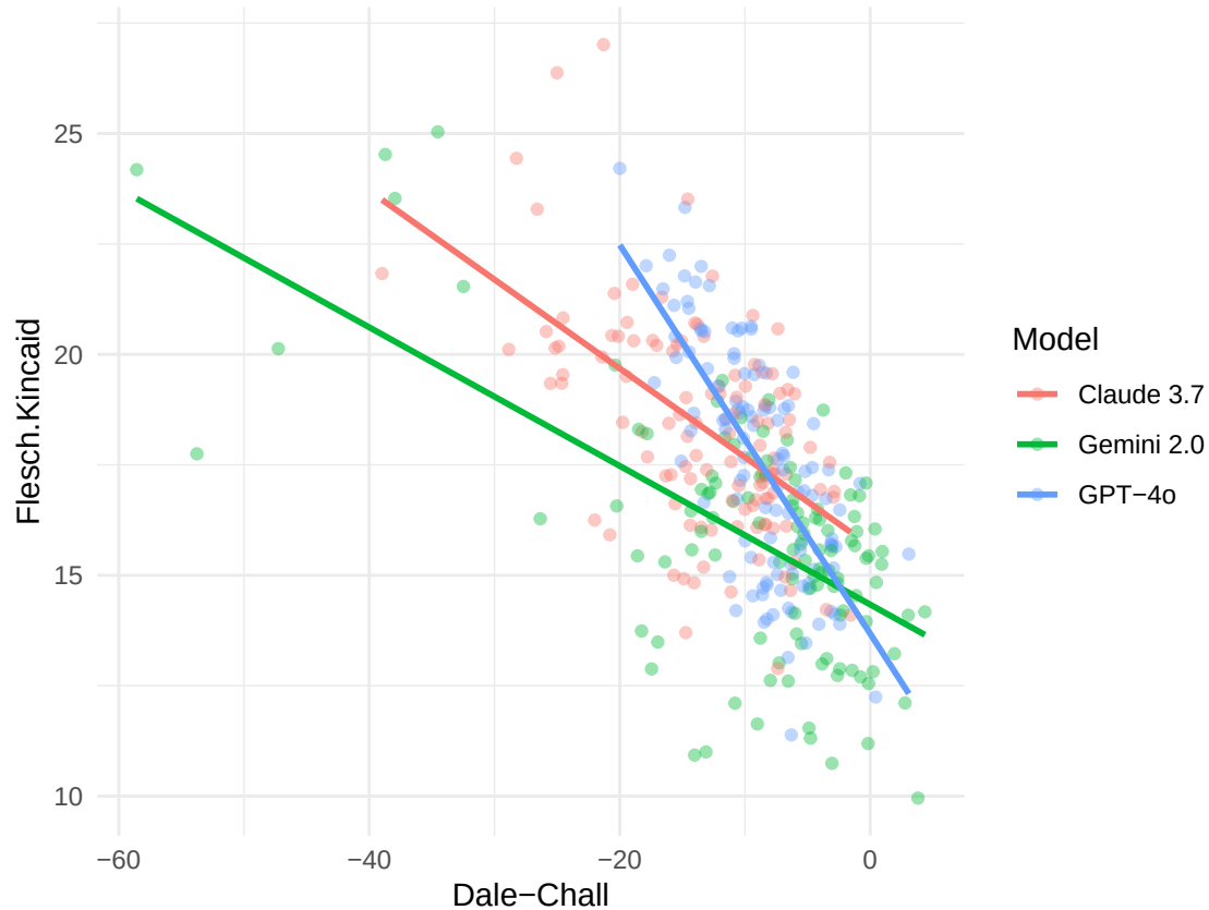
Dale-Chall vs. Flesch.Kincaid per Model
