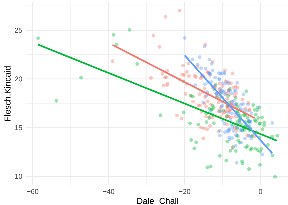
Dale-Chall vs. Flesch.Kincaid per non-reasoning model
