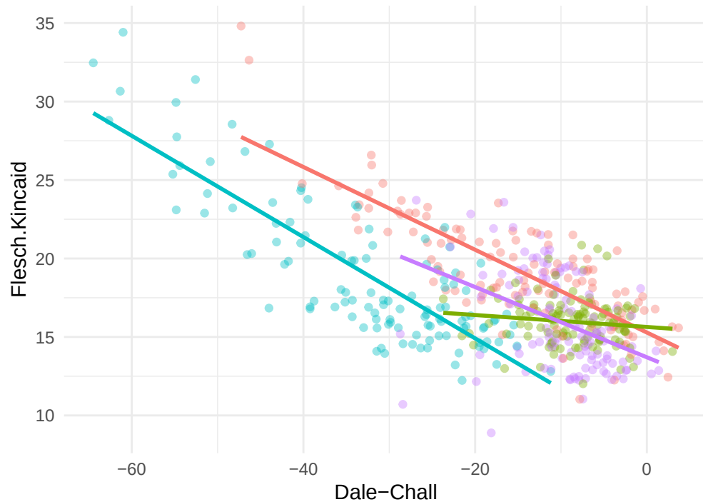
Dale-Chall vs. Flesch.Kincaid per reasoning model
