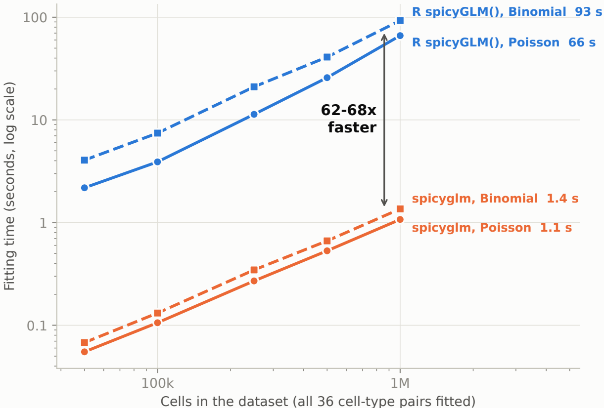
A Faster at every dataset size (synthetic data)
