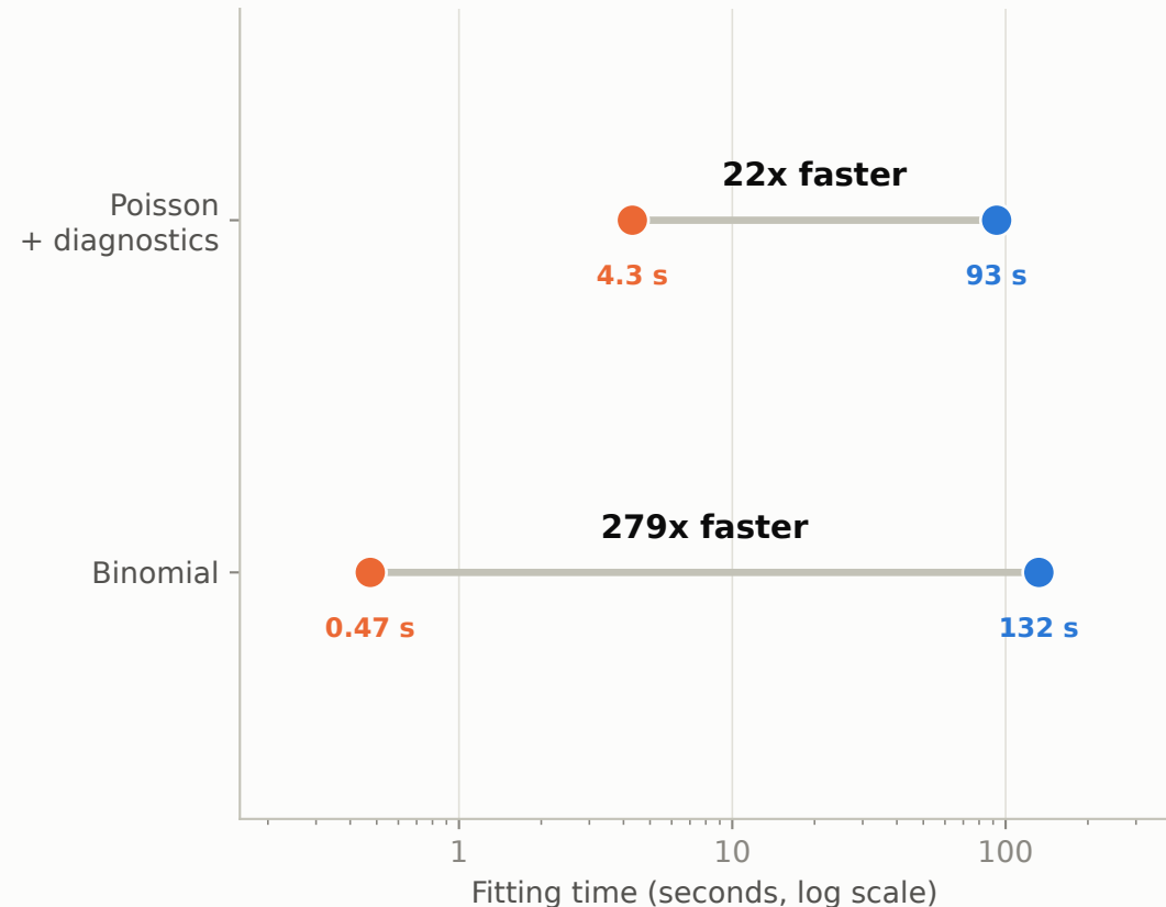
B Real data: Schürch 2020 CRC (258k cells)
