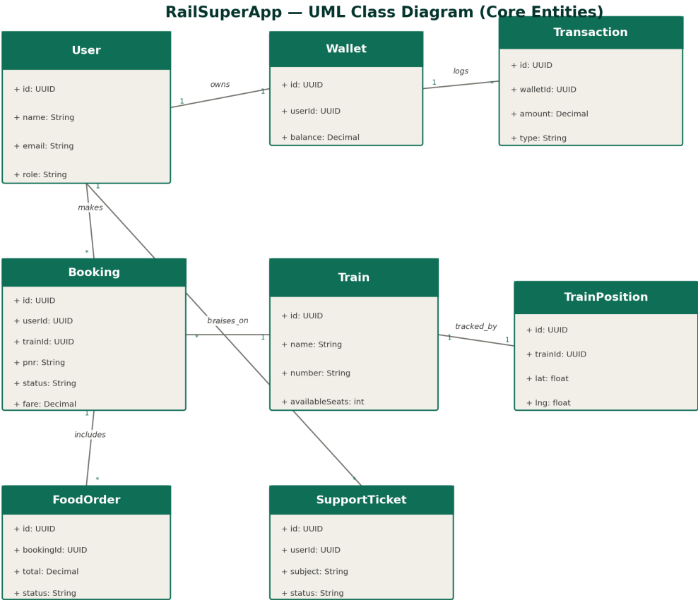
Figure: UML class diagram of RailSuperApp's core domain entities and relationships.
