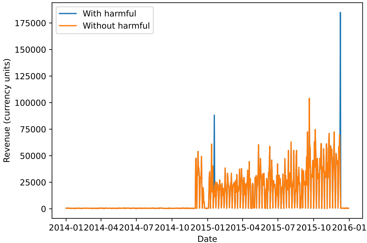
RQ2: Daily revenue trend (with vs without harmful outliers)
