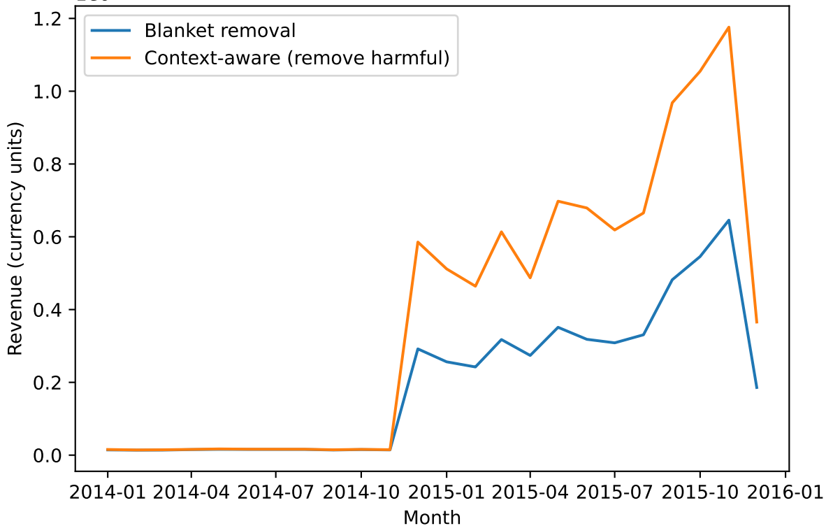
1e6 RQ3: Monthly revenue trend (blanket vs context-aware)
