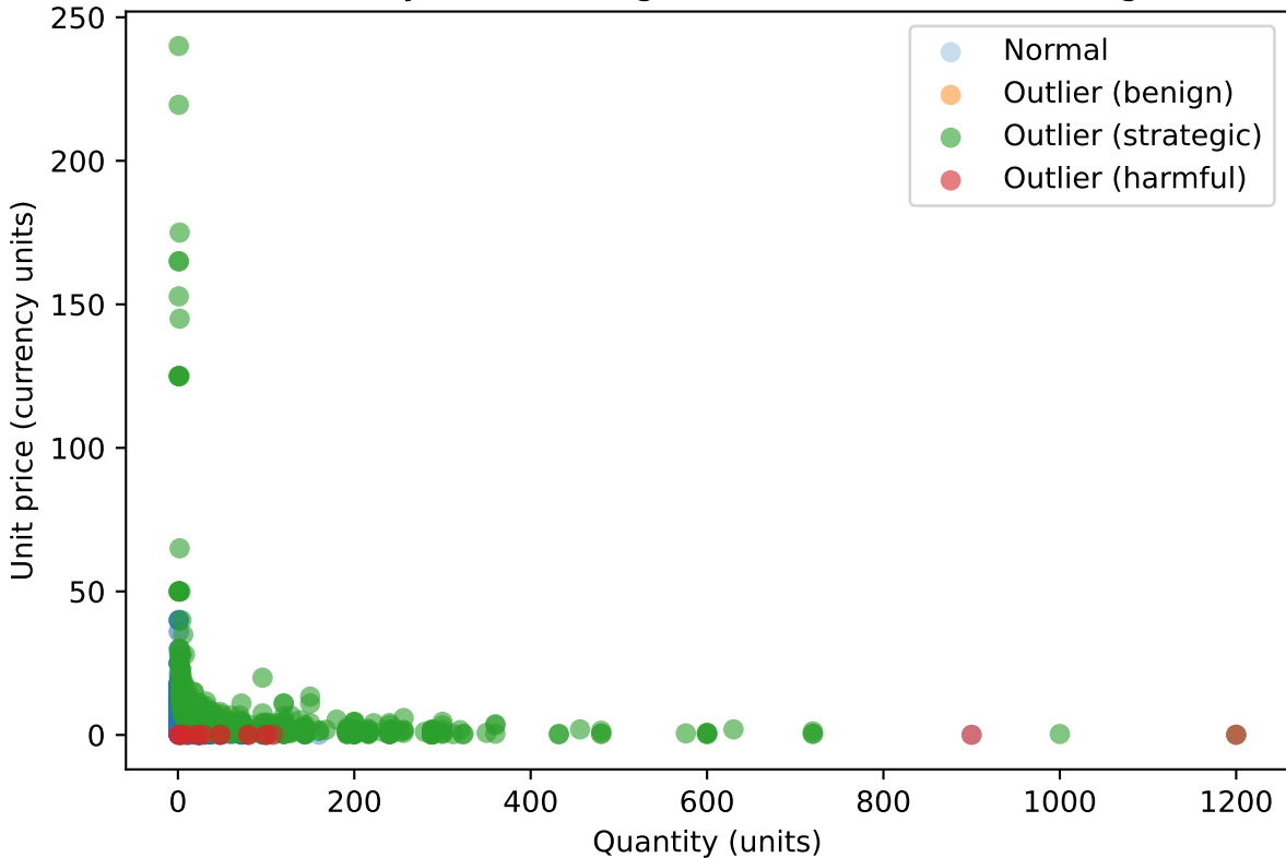
RQ3: Quantity vs Price diagnostic scatter (outlier categories)
