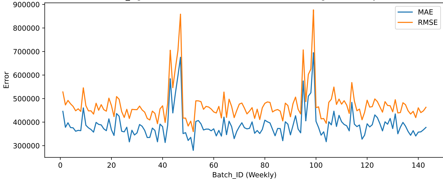
RQ3_Fig1: Forecast Error Metrics Over Time (Rolling Mean Proxy)
