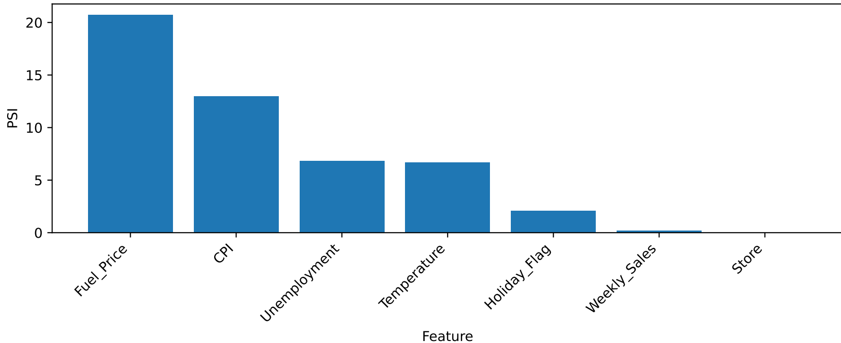
RQ1_Fig2: Top Drifted Features by PSI (Baseline vs New Batch)
