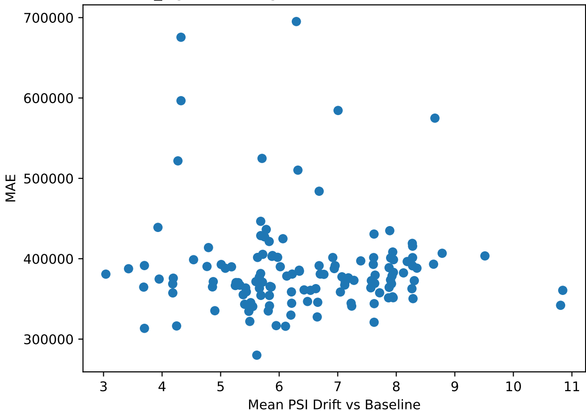
RQ3_Fig2: Drift Magnitude vs MAE (Pearson r=-0.043 )
