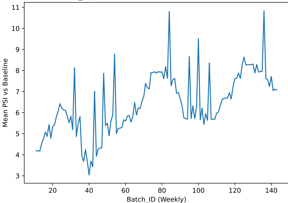
RQ1_Fig3: Drift Trend Across Batches (Mean PSI)
