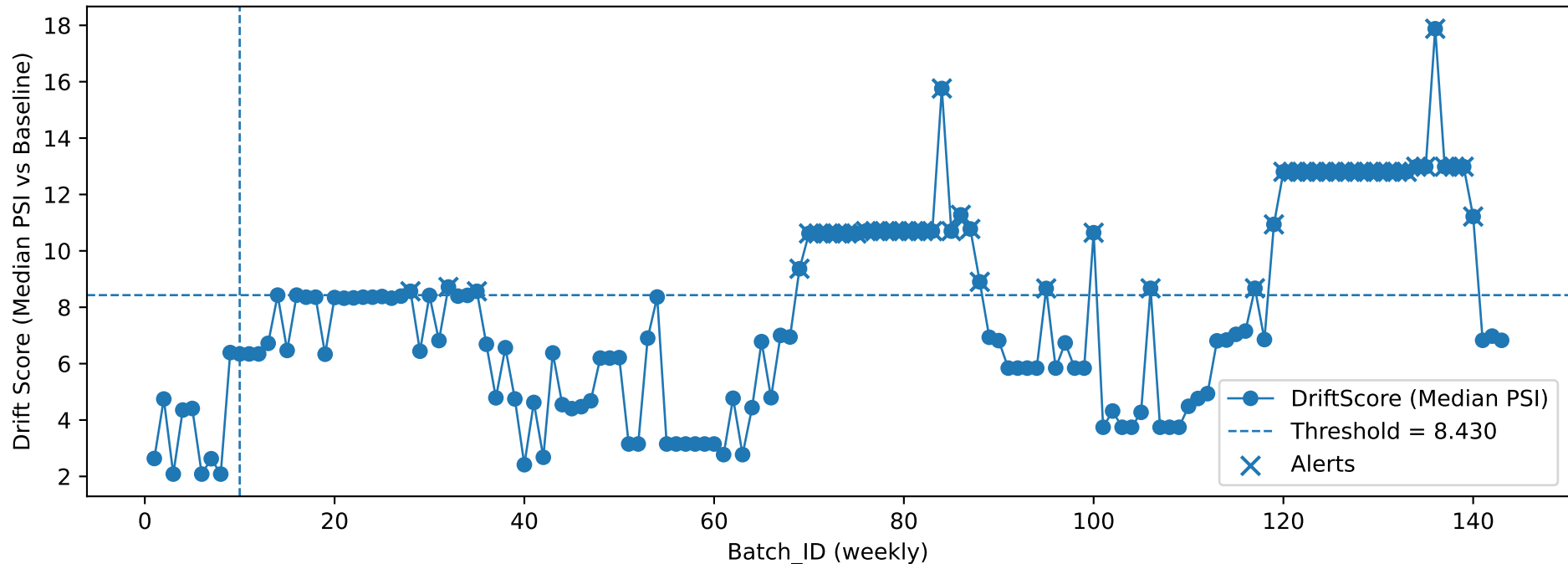
RQ4_Fig2: Drift Trend and Alert Threshold (WarmupQuantile(target=10%))
