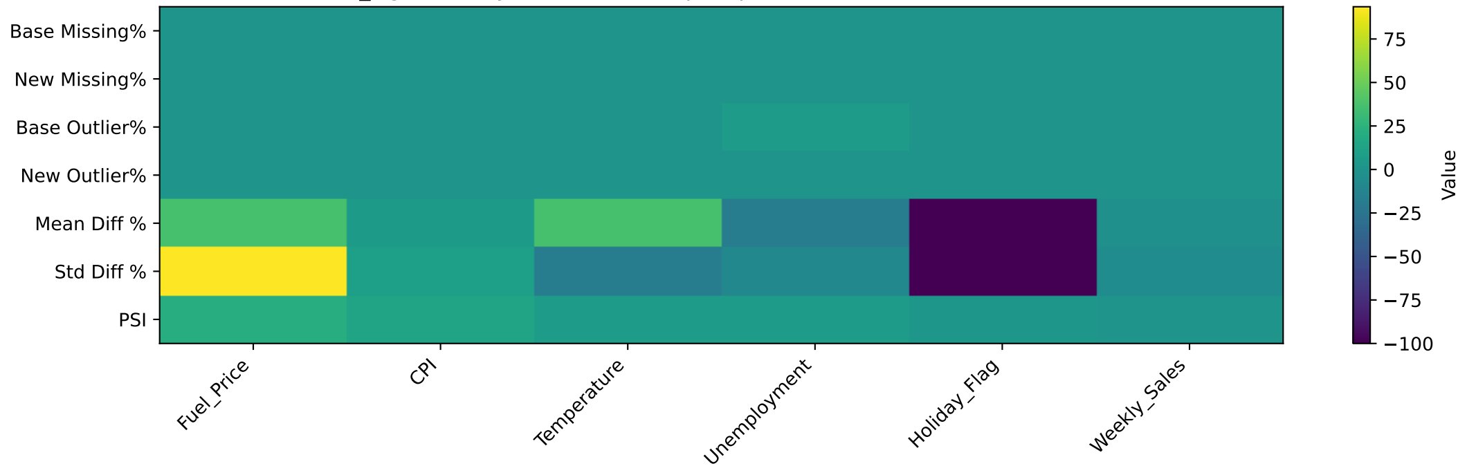
RQ2_Fig1: Quality + Drift Heatmap (Top Columns, Baseline vs New Batch)
