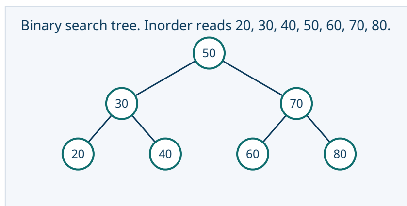
Figure 10. Left child smaller, right child larger. Inorder of this tree is sorted.
