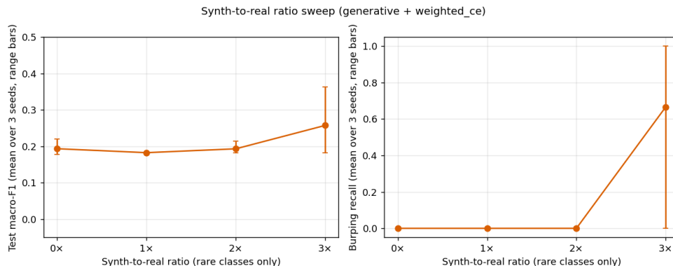
Figure 4: Synth-to-real ratio sweep (generative + weighted_ce). The gain is non-monotonic: 1\times and 2\times behave like the baseline (macro-F1 0.18–0.19; no burping recovery), but 3\times crosses an argmax threshold and the burping recall jumps from 0 to 0.667. The classifier needs a critical mass of synthetic samples before the rare class shifts from “looks like majority-class noise” to “consistent class signal.”
