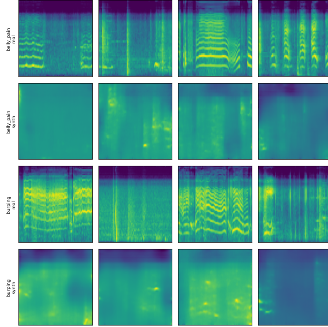
Figure 1: Real vs. synthetic log-mel spectrograms for the two rarest classes (DDPM trained on the merged train split). The class-consistency probe identifies 93% of synthetic belly_pain samples as belly_pain and 8% of synthetic burping samples as burping .
