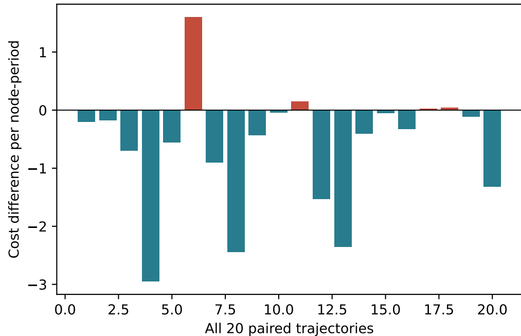
Fixed LLM library + screen minus Frozen HAPPO (seed 11, k=3)
