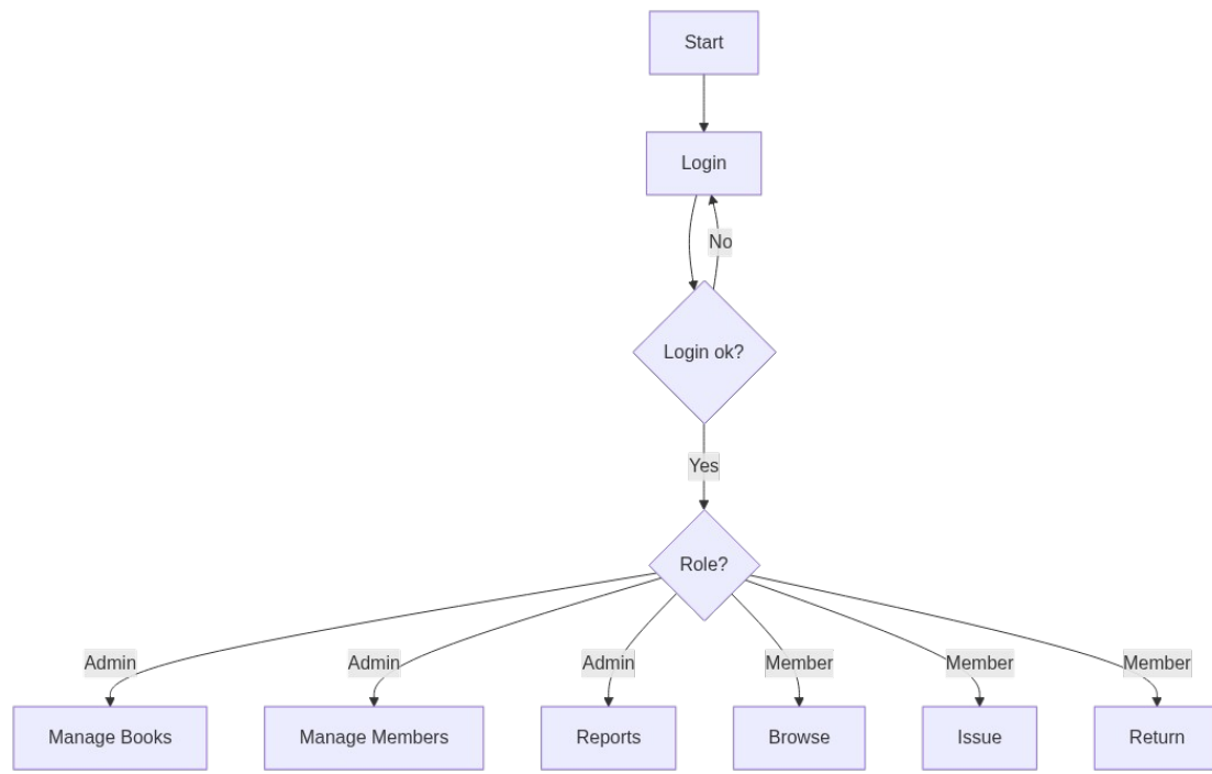
Screenshot of flowchart TD diagram
