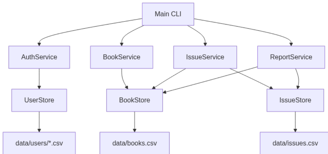
Screenshot of graph TD diagram
