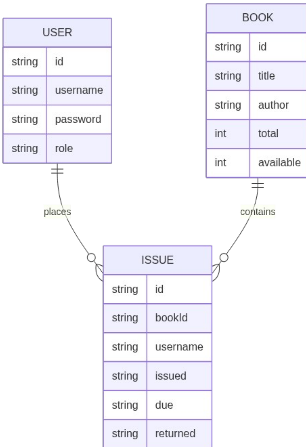
Screenshot of erDiagram diagram
