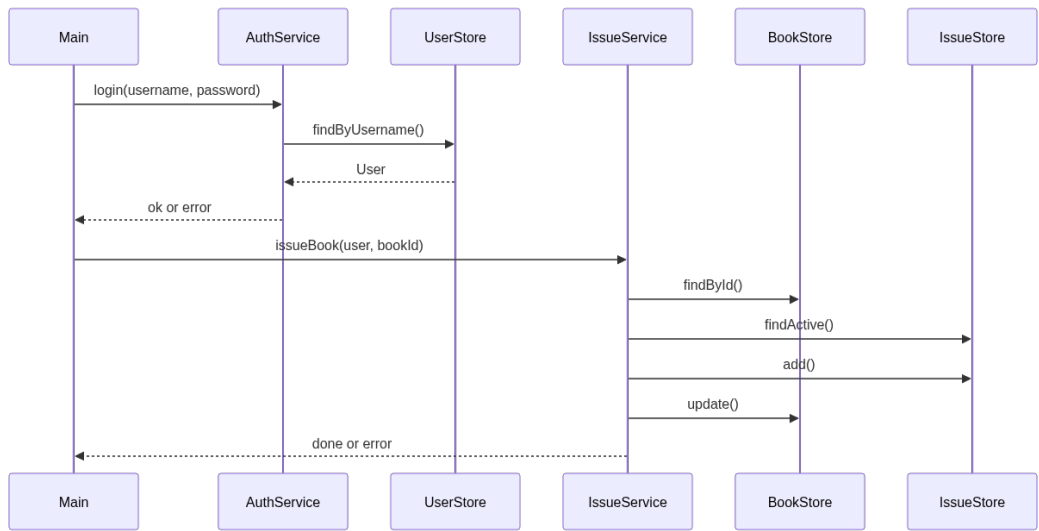
Screenshot of sequenceDiagram diagram
