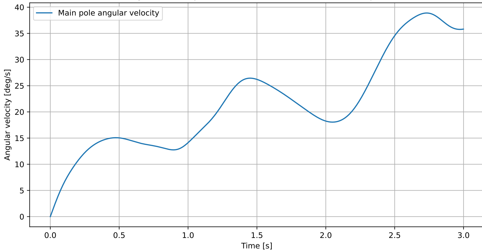
Angular velocity around the vertical axis of the main pole
