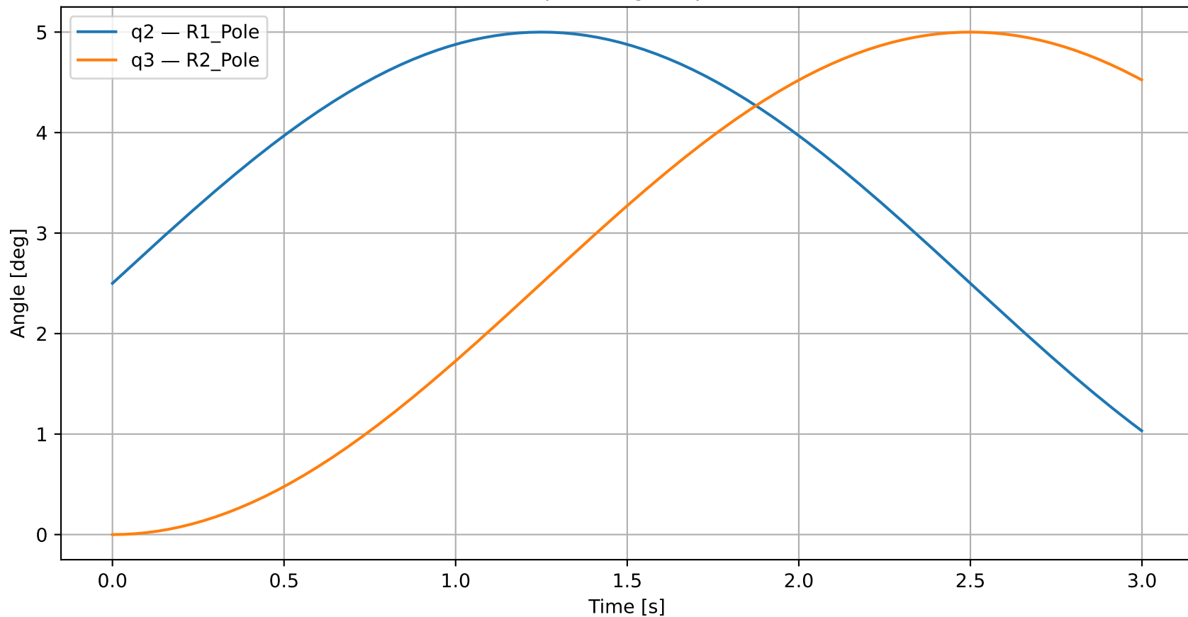
Driven joint angles (pole tilt)
