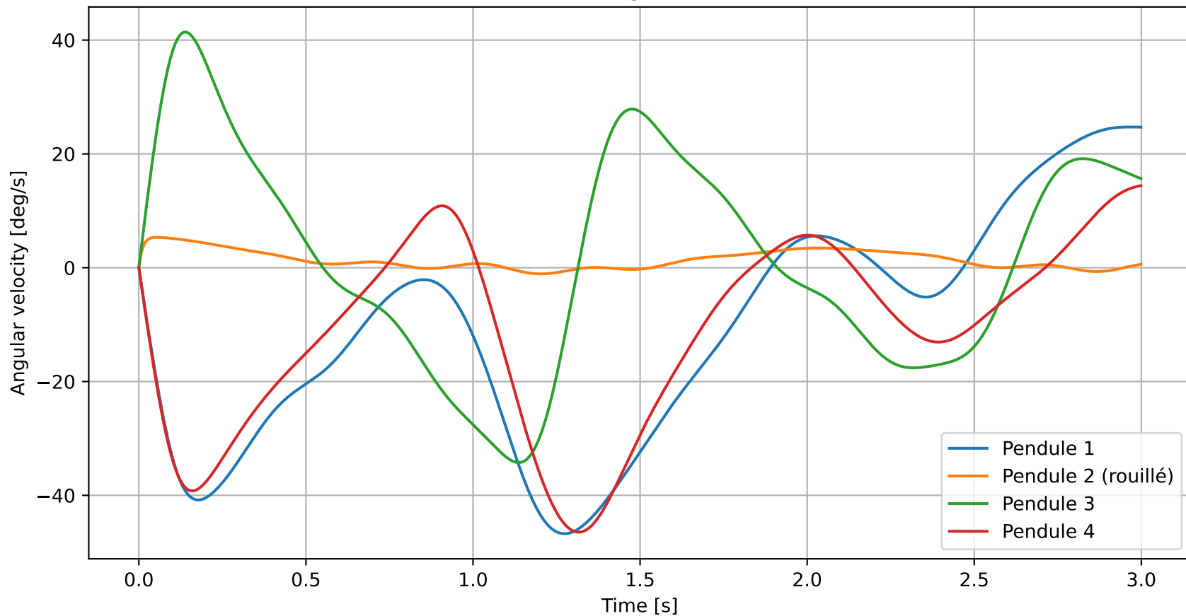
Pendulum angular velocities
