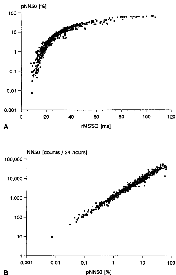
Figure 1. Relationship between the rMSSD and pNN50 (panel A), and pNN50 and NN50 (panel B) measures of HRV assessed from 857 nominal 24-hour Holter tapes recorded in survivors of acute myocardial infarction prior to hospital discharge. The NN50 measure, used in panel B, was normalized in respect to the length of the recording (Data of St. George's Post-infarction Research Survey Programme.)
