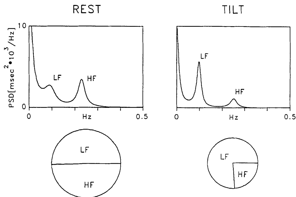
Figure 3. Spectral analysis (autoregressive model, order 12) of RR interval variability in a healthy subject at rest and during 90° head up tilt. At rest, two major components of similar power are detectable at low and high frequencies. During tilt, the LF component becomes dominant but, as total variance is reduced, the absolute power of LF appears unchanged compared to rest. Normalization procedure leads to predominant LF and smaller HF components which express the alteration of spectral components due to tilt. The pie charts show the relative distribution together with the absolute power of the two components represented by the area. During rest, the total variance of the spectrum was 1201 ms 2 , and its VLF, LF, and HF components were 586 ms 2 , 310 ms 2 , and 302 ms 2 , respectively. Expressed in normalized units (n.u.), the LF and HF were 48.95 n.u. and 47.78 n.u., respectively. The LF/HF ratio was 1.02. During tilt, the total variance was 671 ms 2 , and its VLF, LF, and HF components were 265 ms 2 , 308 ms 2 , and 95 ms 2 , respectively. Expressed in normalized units, the LF and HF were 75.96 n.u. and 23.48 n.u., respectively. The LF/HF ratio was 3.34. Thus note that, for instance, the absolute power of the LF component was slightly decreased during tilt while the normalized units of LF were substantially increased.
