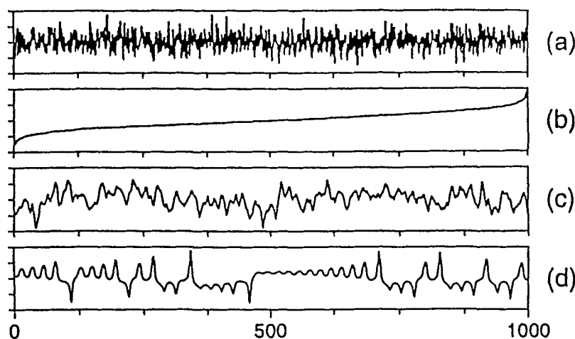
Figure 6. Example of four synthesized time series with identical means, standard deviations, and ranges. Series (c) and (d) also have identical autocorrelation functions and therefore identical power spectra. (Reprinted with permission. 39 )
