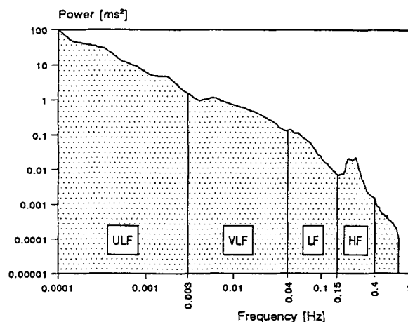
Figure 4. Example of an estimate of power spectral density obtained from the entire 24-interval of a long-term Hoiter recording. Only the LF and HF components correspond to peaks of the spectrum while the VLF and ULF can be approximated by a line in this plot with logarithmic scales on both axes. The slope of such a line is the \alpha measure of HRV.
