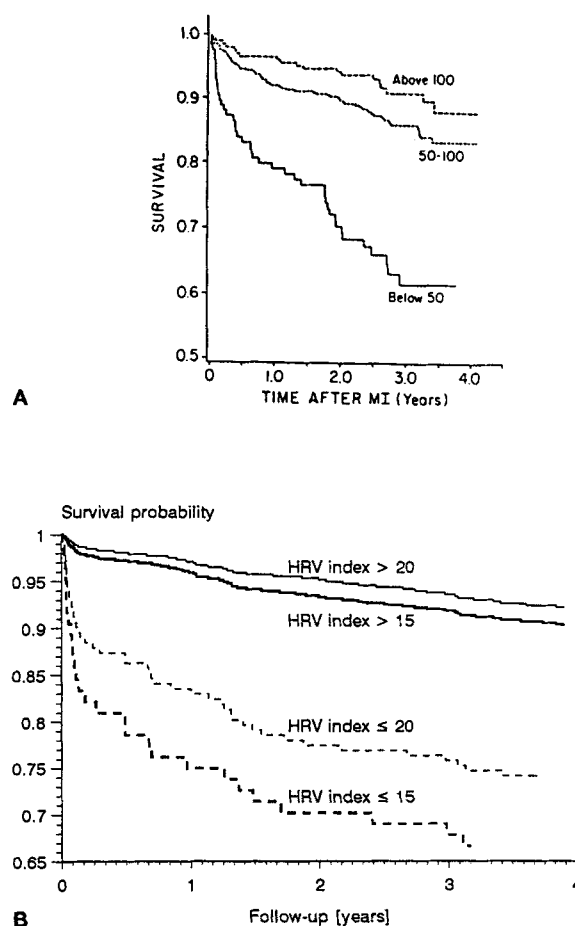
Figure 8. Cumulative survival of patients after MI. Panel A shows survival of patients stratified according to 24-hour SDNN values into 3 groups with cut-off points of 50 and 100 ms. (Reprinted with permission. 16 ) Panel B shows similar survival curves of patients stratified according to 24-hour HRV triangular index values with cut-off points of 15 and 20 units, respectively. (Data of St. George's Post-infarction Research Survey Programme.)
