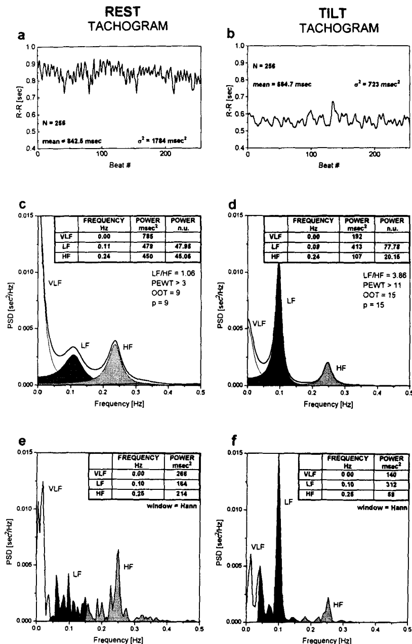
Figure 5. Interval tachogram of 256 consecutive RR values in a normal subject at supine rest (panel a) and after head-up tilt (panel b). The HRV spectra are shown, calculated by parametric autoregressive modeling (panels c and d), and by a FFT based non-parametric algorithm (panels e and f). Mean values (m), variances ( s^2 ) and the number N of samples are indicated. For (panels c and d), VLF, LF and HF central frequency, power in absolute value and power in normalized units (n.u.) are also indicated together with the order p of the chosen model and minimal values of PEWT and OOT which satisfy the tests. In panels e and f, the peak frequency and the power of VLF, LF and HF were calculated by integrating the PSD in the defined frequency bands. The window type is also specified. In panels c–f, the LF component is indicated by dark shaded areas and the HF component by light shaded areas.
