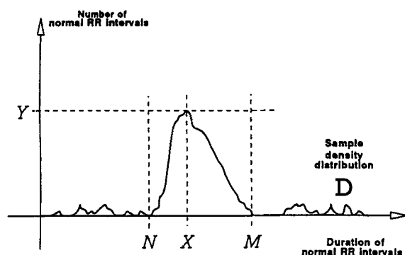
Figure 2. To perform geometrical measures on the NN interval histogram, the sample density distribution D is constructed which assigns the number of equally long NN intervals to each value of their lengths. The most frequent NN interval length X is established, that is Y = D(X) is the maximum of the sample density distribution D . The HRV triangular index is the value obtained by dividing the area integral of D by the maximum Y . When constructing the distribution D with a discrete scale on the horizontal axis, the value is obtained according to the formula: HRV index = (total number of all NN intervals)/ Y . For the computation of the TINN measure, the values N and M are established on the time axis and a multilinear function q constructed such that q(t) = 0 for t \leq N and t \geq M and q(X) = Y , and such that the integral \int_0^{+\infty} (D(t) - q(t))^2 dt is the minimum among all selections of all values N and M . The TINN measure is expressed in milliseconds and given by the formula TINN = M - N .
