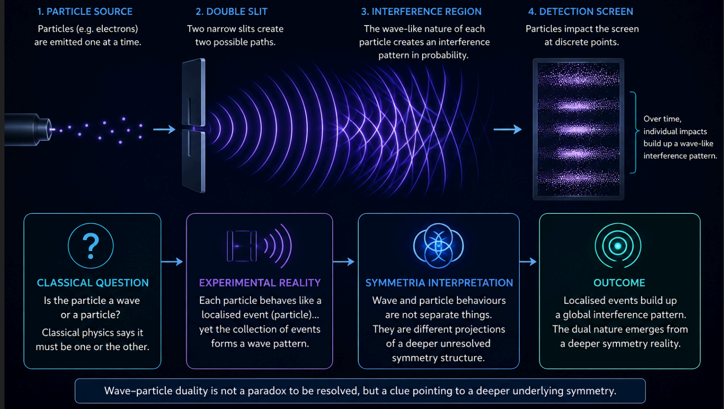
Figure 1.1: Wave-particle duality shown through the double-slit experiment. Individual quantum events arrive as localised particle impacts, yet over time they build a wave-like interference pattern. In the SYMMETRIA interpretation, the apparent contradiction arises because both wave and particle behaviour are projected expressions of a deeper unresolved symmetry structure.
