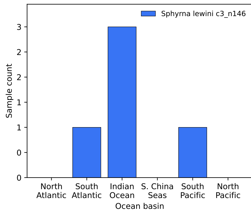
Sphyrna lewini c3_n146
