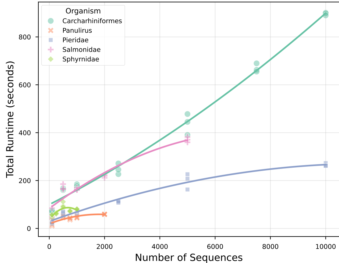
A. Runtime Scaling
