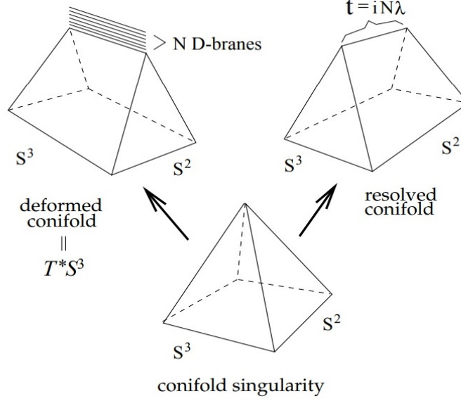
A local representation of the geometric transition between the deformed and resolved conifold. Taken from [21].
