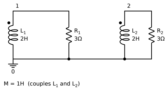
Figure B.6: The coupled coils with an initial current (§5.6).
