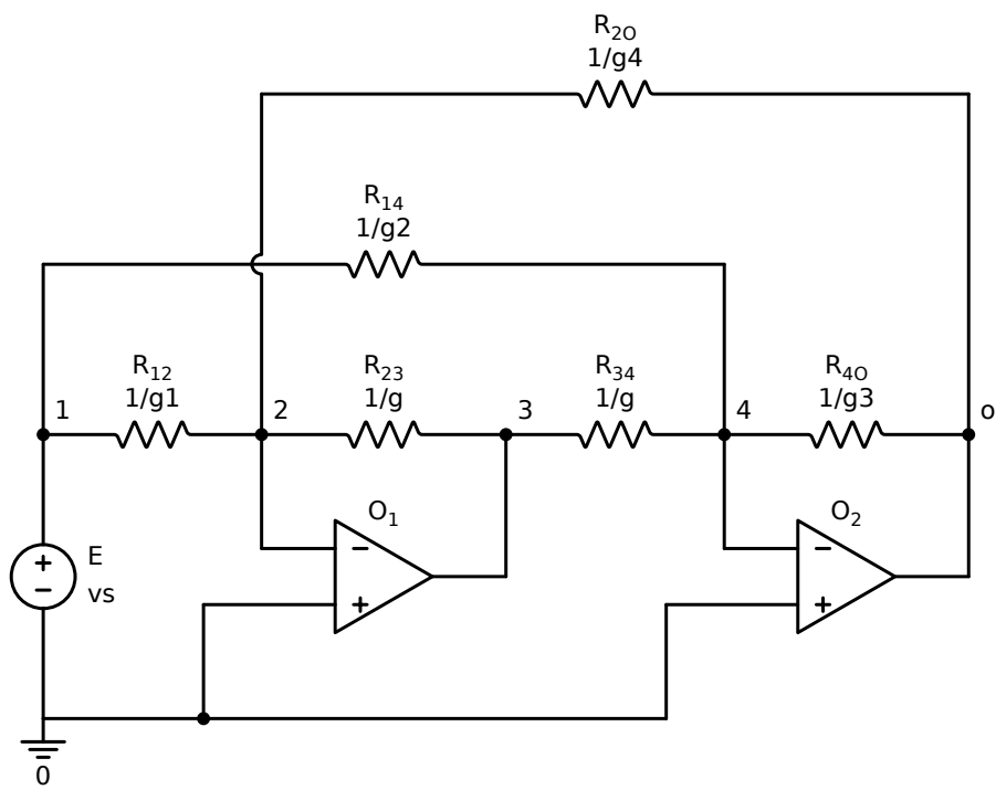
Figure B.7: The all-symbolic two-op-amp cascade (§5.7).
