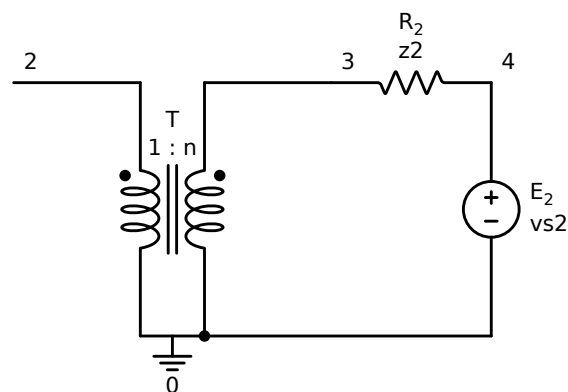
Figure B.5: The ideal transformer viewed from its primary (§5.5), every value a symbol.
