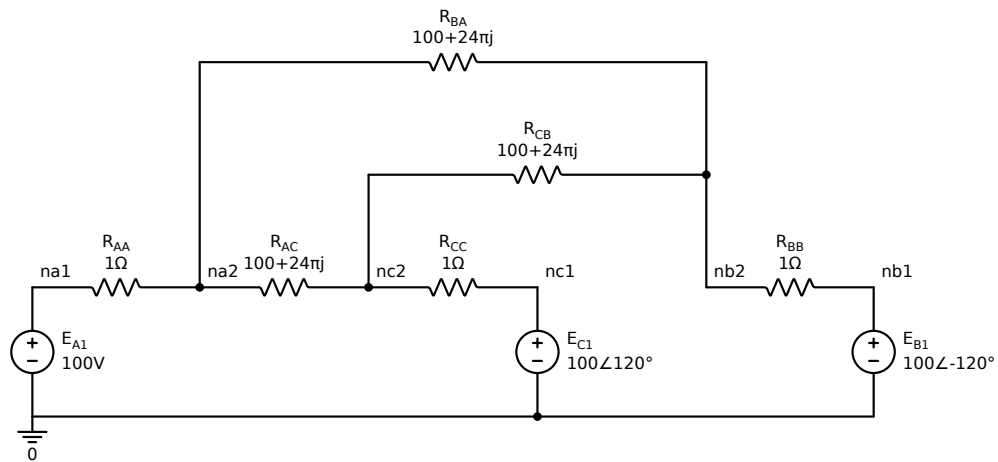
Figure B.4: The balanced wye-delta system with line impedances (§5.4), its sources typed in angle notation.
