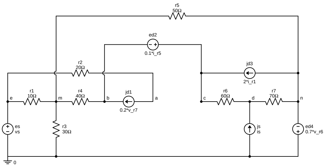
Figure B.2: The 2013 showcase (§5.2): one dependent source of each species, and both independent sources symbolic.
