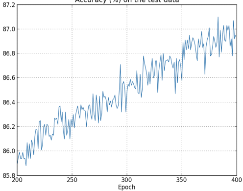
Accuracy (%) on the test data
