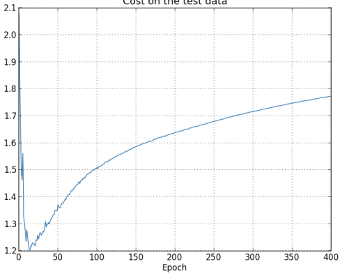
Cost on the test data
