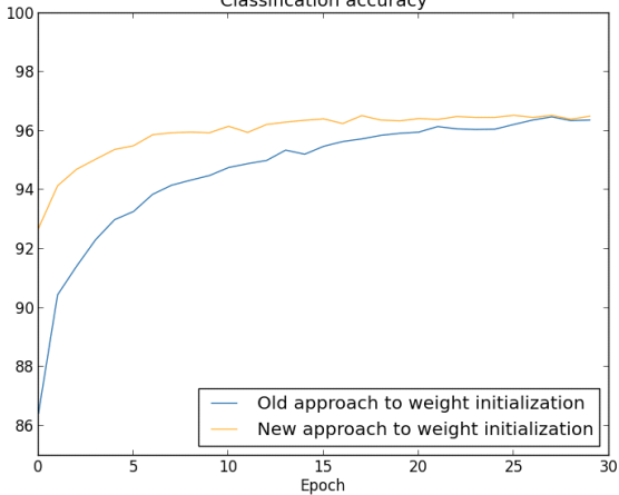
Classification accuracy
