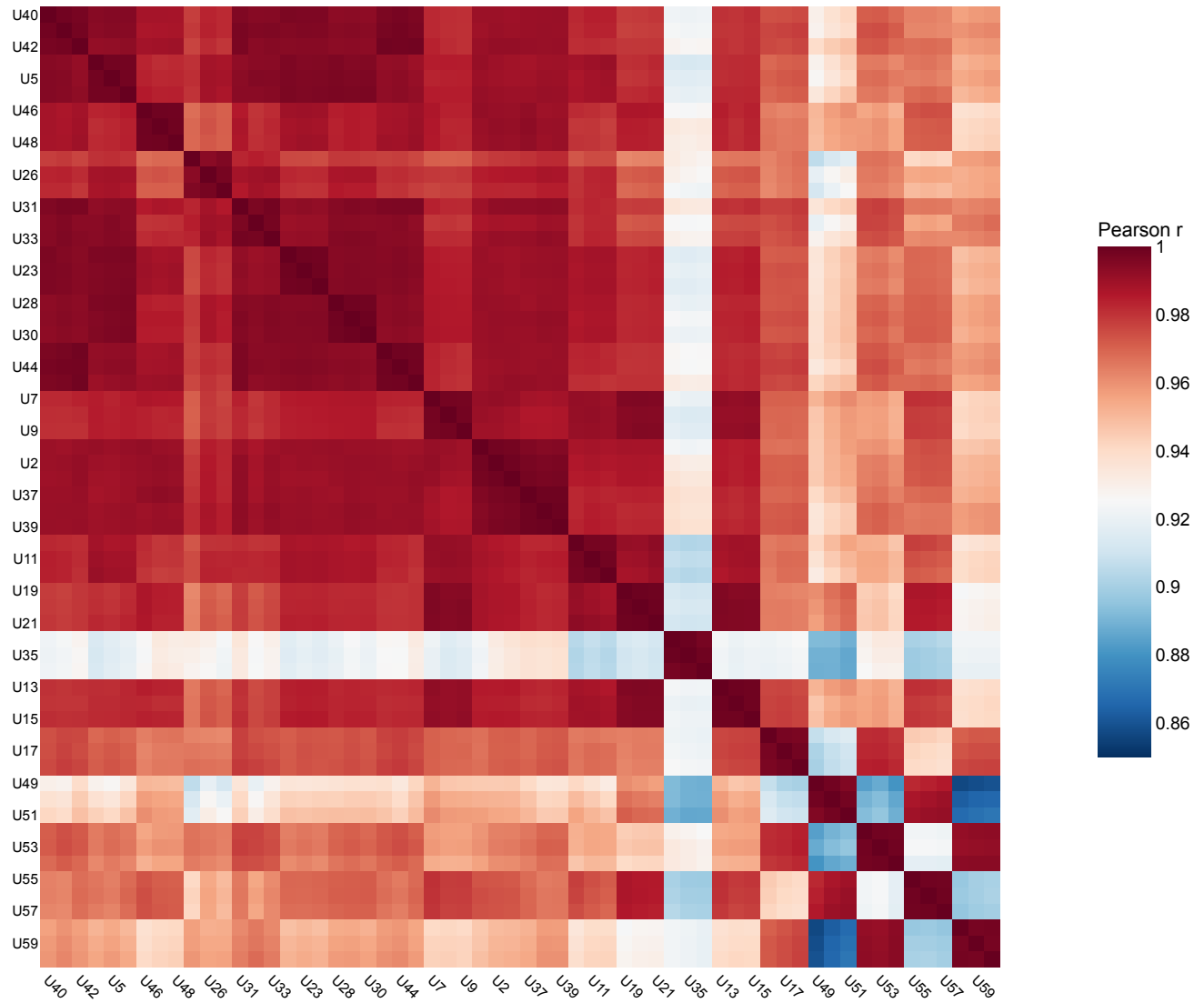
Sample Correlation Matrix
