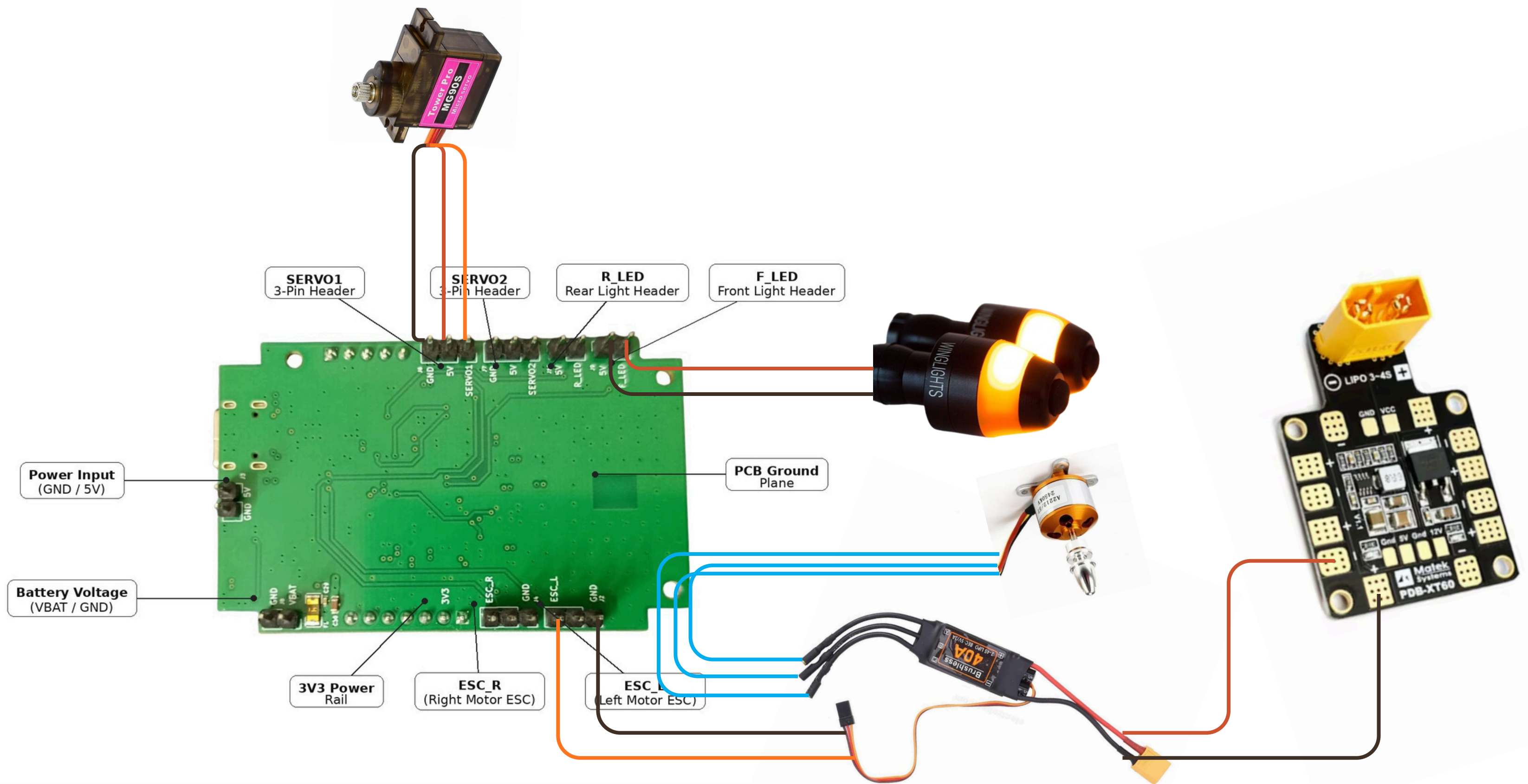
RX Boat PCB — Bottom View (Connectors)
