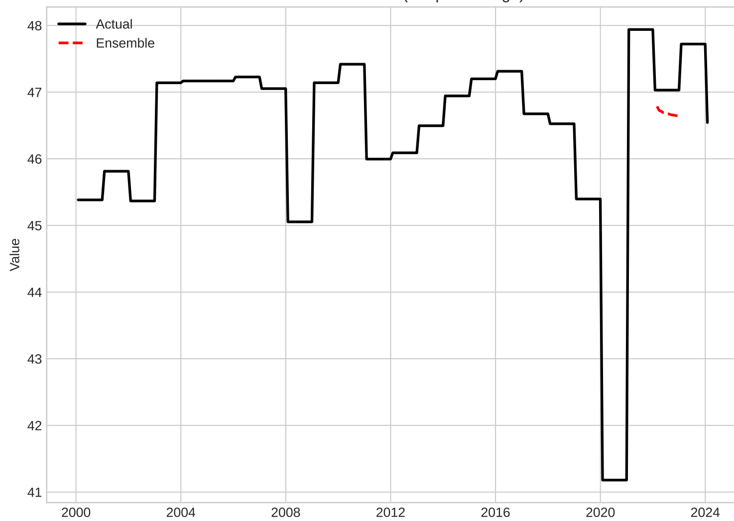
Ensemble Forecast (Simple Average)
