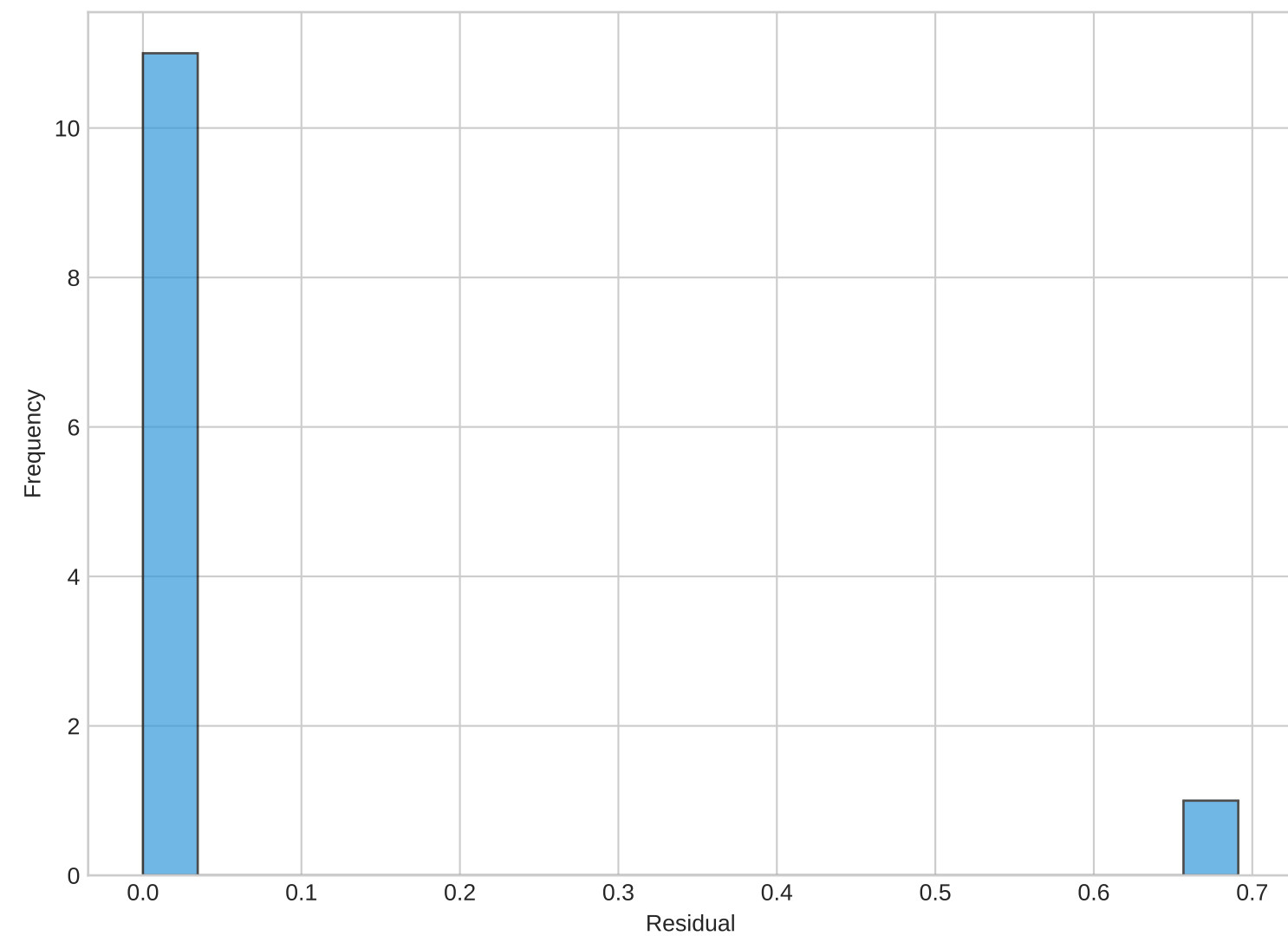
SARIMAX Residuals Distribution
