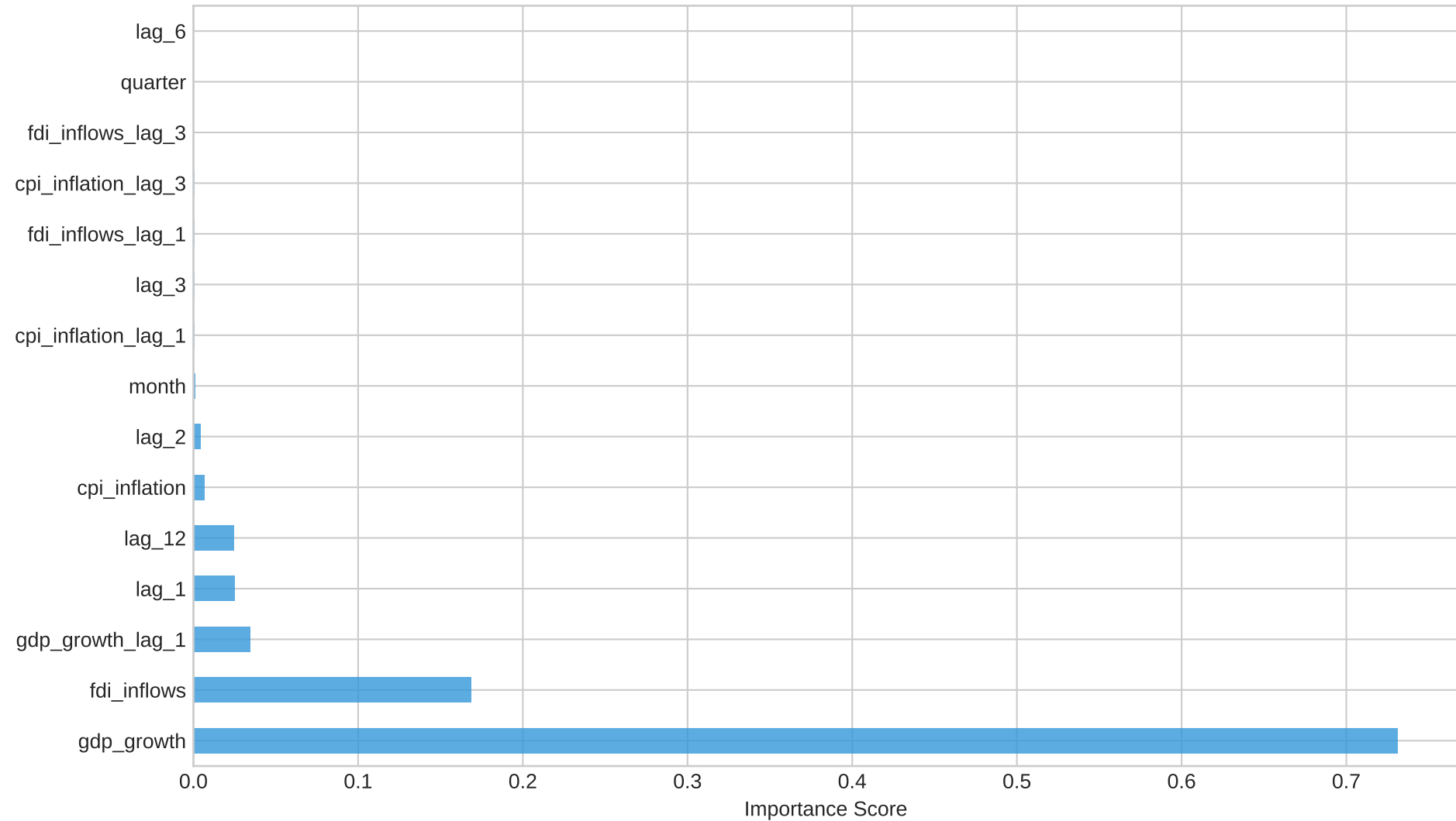
XGBoost Feature Importance (Top 15)
