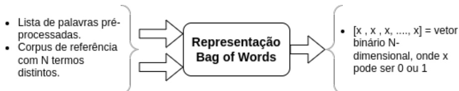
Figura 3: Modelagem bag of words.
