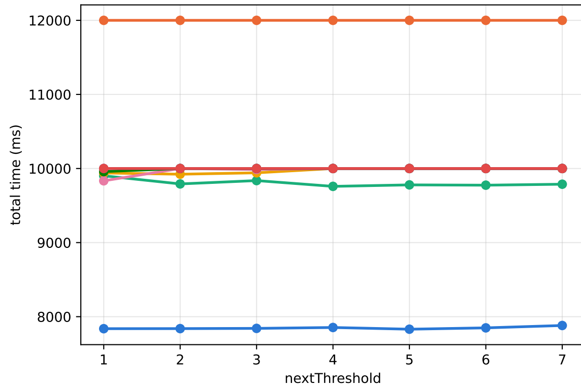
Total ClauseMatcher::next time
