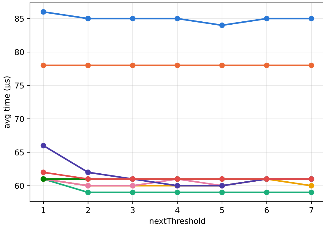
Avg time per ClauseMatcher::next call
