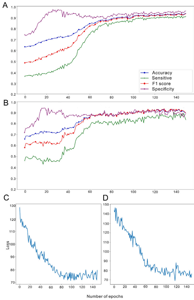
Fig. 7. (A) Curves of relevant parameters in the training process corresponding to the CHB-MIT dataset. (B) Curves of relevant parameters in the training process corresponding to the Siena scalp dataset. (C) The loss value change curve of the CHB-MIT dataset during the training process. (D) The loss value change curve of the Siena scalp dataset during the training process.
