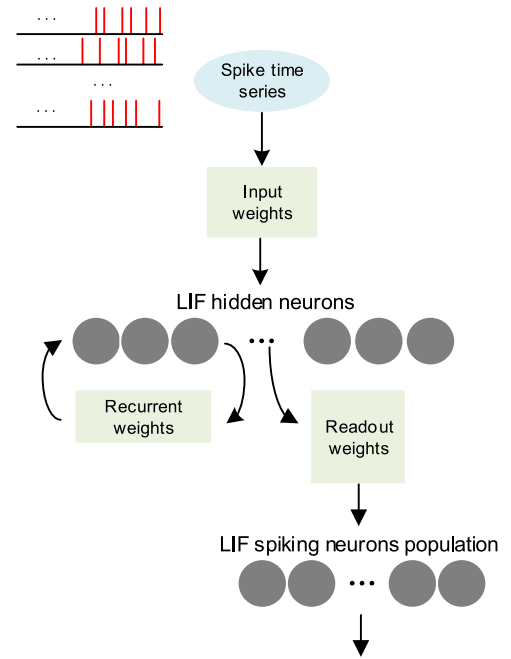
Fig. 3. Xylo comprises a hidden population of 1000 LIF neurons and a readout population of 8 LIF neurons. Dense input and output weights are available, along with sparse recurrent weights that can target up to 32 hidden neurons per neuron. The inputs, which consist of 16 channels, and the outputs, which consist of 8 channels, are transmitted through asynchronous firing events.
