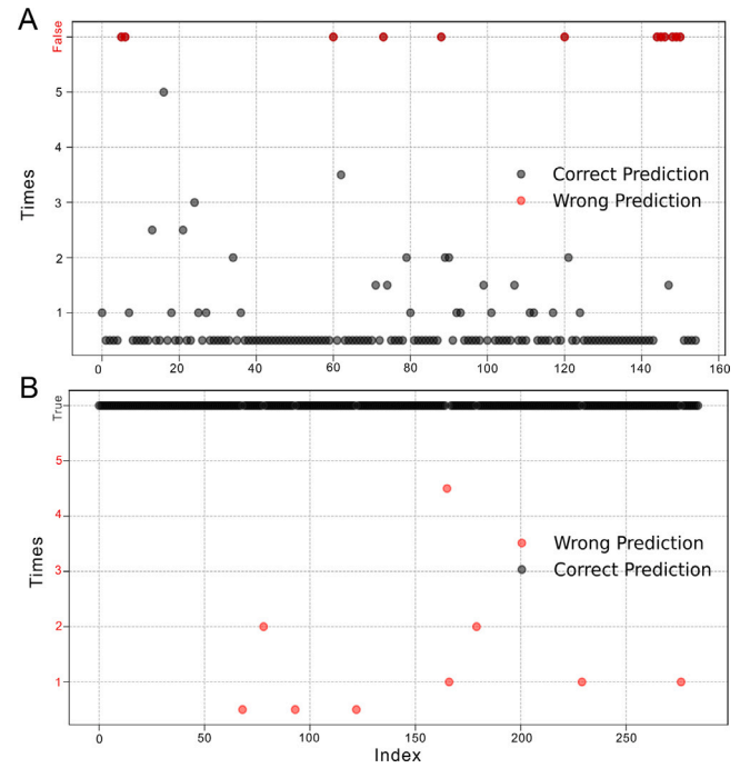
Fig. 8. (A) Latency test results for partially positive samples. The black dot's vertical axis value signifies the accurate prediction time of epilepsy, while the red dot indicates that the model failed to detect epilepsy even after surpassing the corresponding sample time. (B) Latency test results for partial negative samples. The red dot signifies that the model wrongly classified a non-epileptic signal as an epileptic signal at the corresponding time on the y-axis. The black dot denotes that the model accurately classified the signal as non-epileptic even after the sampling time for the sample has passed.
