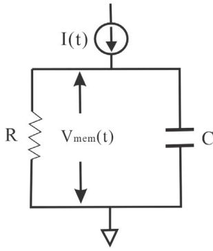
Fig. 1. Equivalent circuit of the LIF neuron model.
