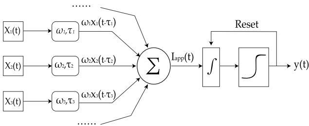
Fig. 2. Block diagram of a Leaky integration and Fire spiking neuron.
