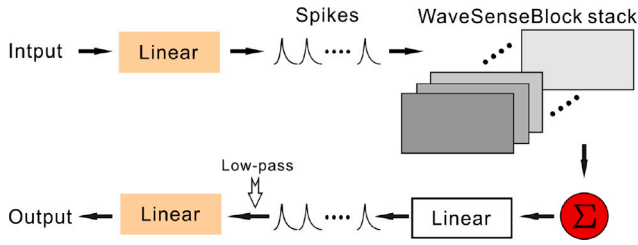
Fig. 6. Overview of the entire architecture.
