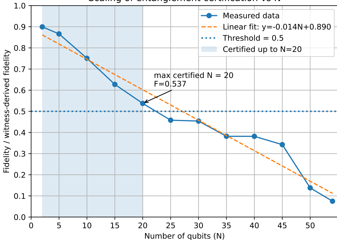
Scaling of entanglement certification vs N
