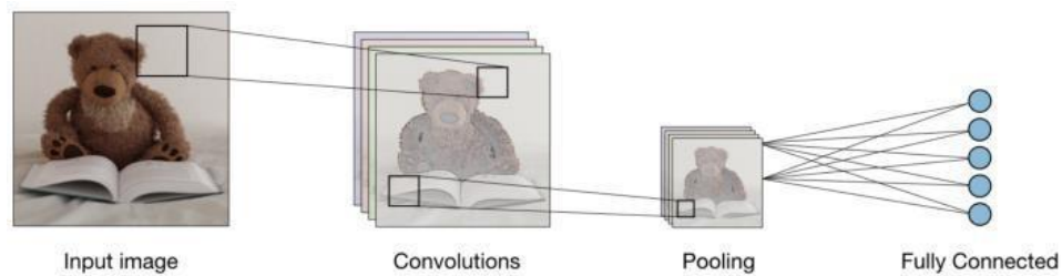
Figure 7: Data flattening into a feed-forward neural
