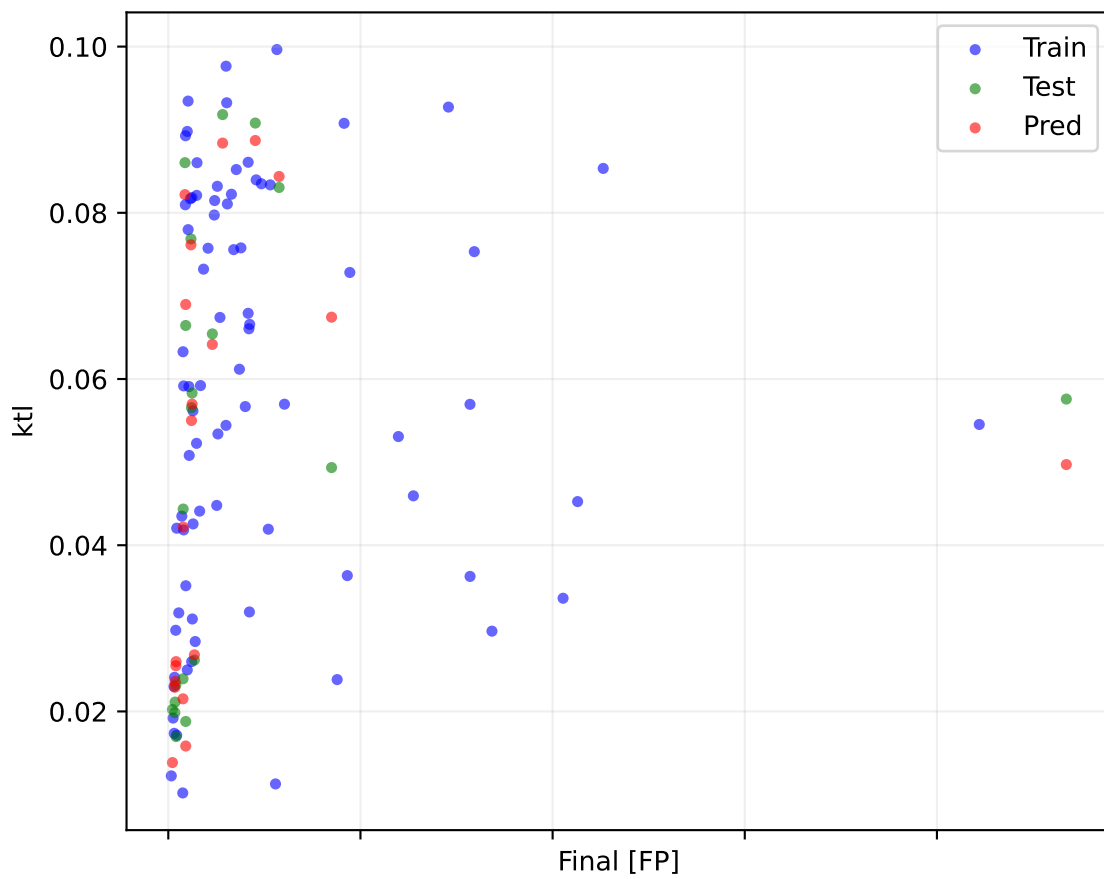
PILSTM Epoch 6000
