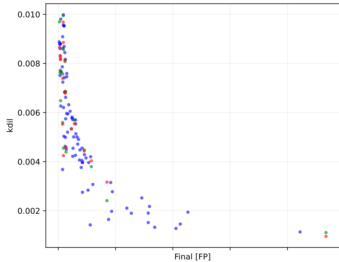
PILSTM Epoch 6000
