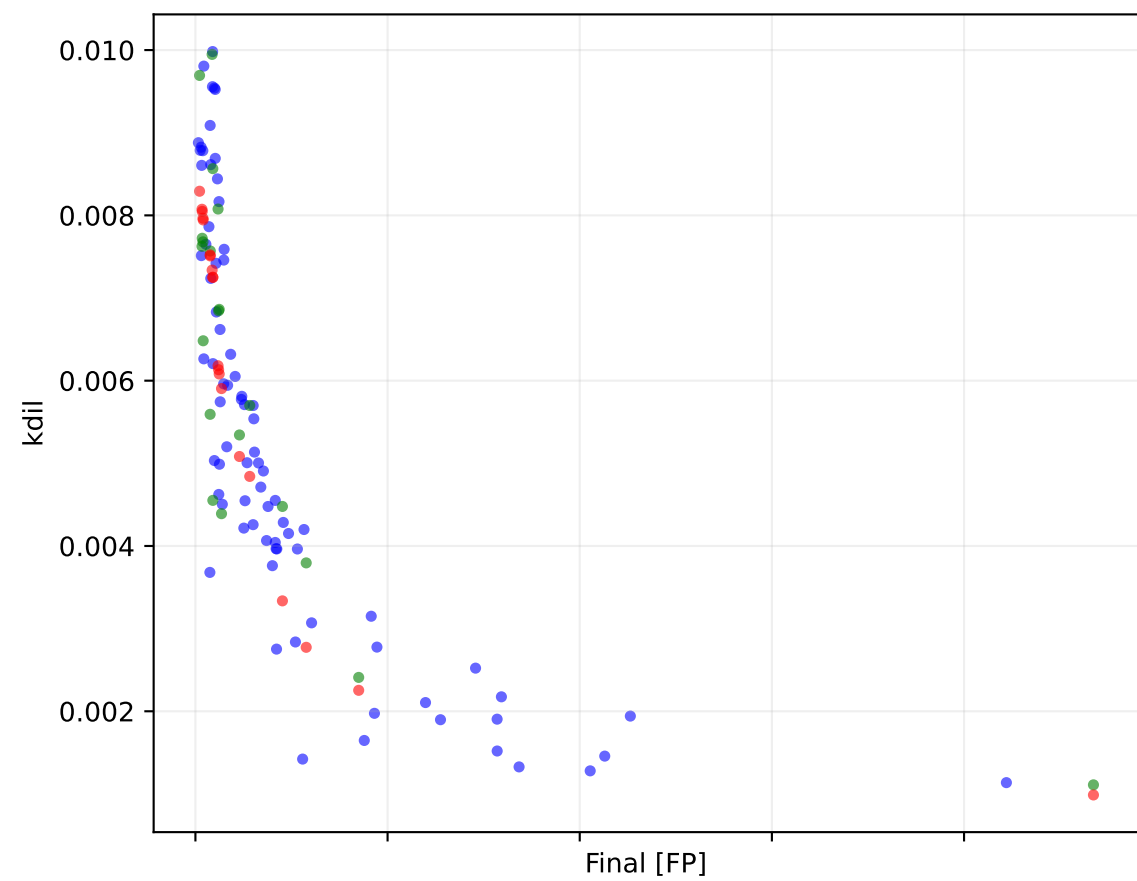
PILSTM Epoch 1000 lambda physics 0.0000
