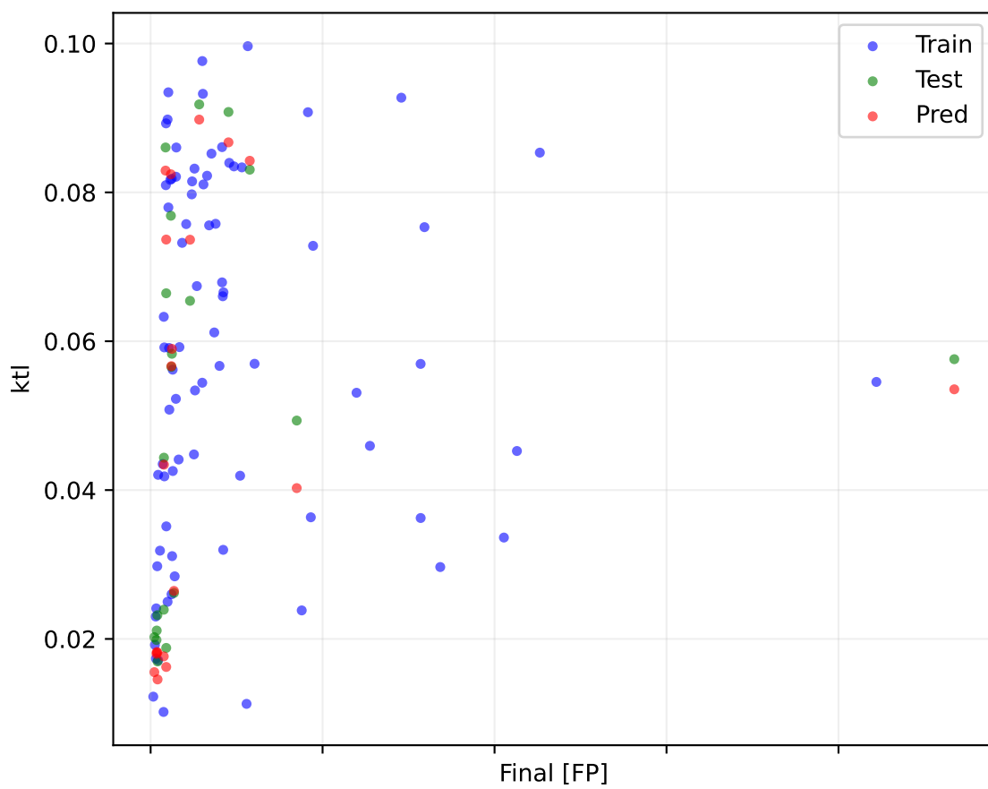
PILSTM Epoch 13000 lambda physics 0.0000
