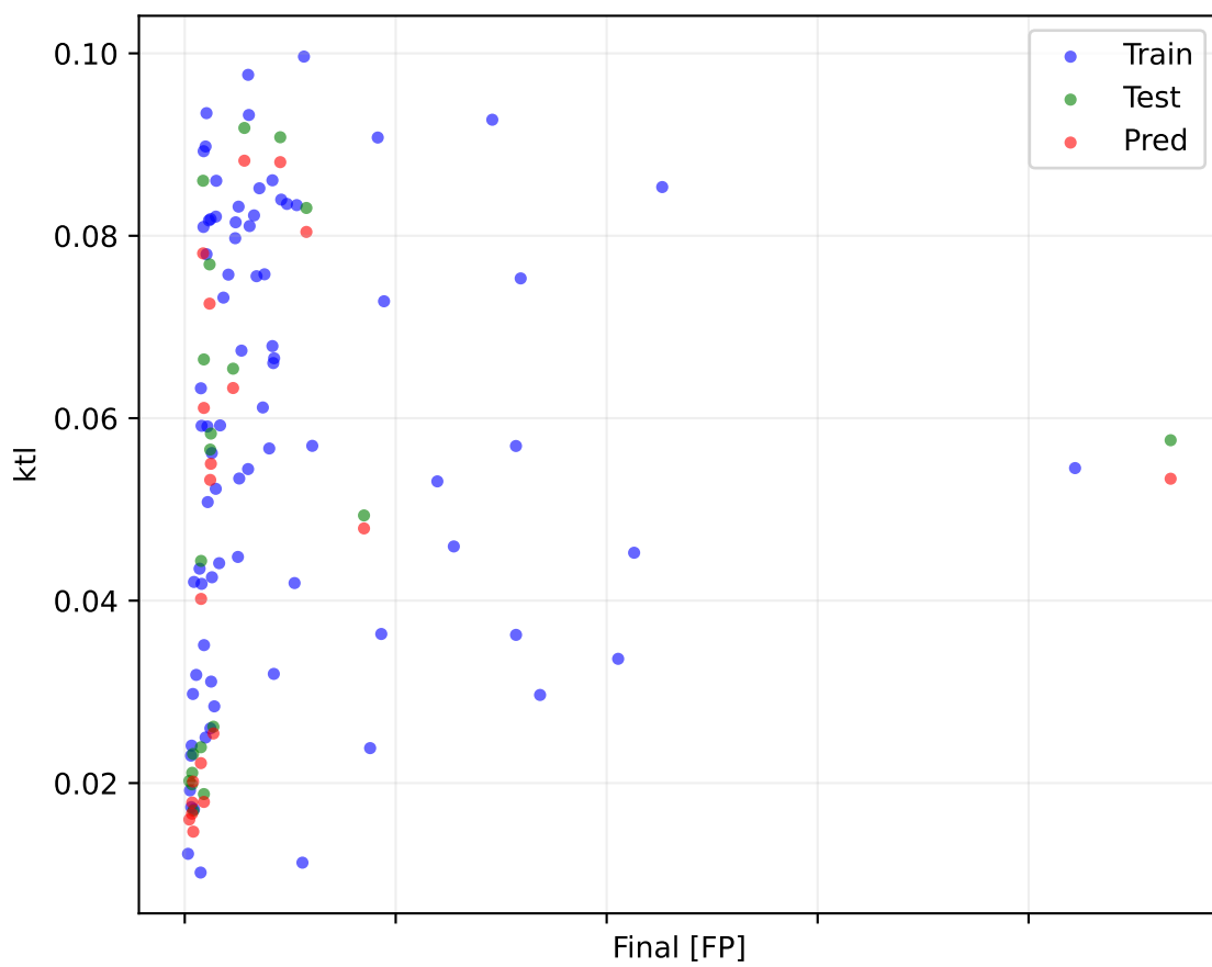
PILSTM Epoch 14000 lambda physics 0.0050
