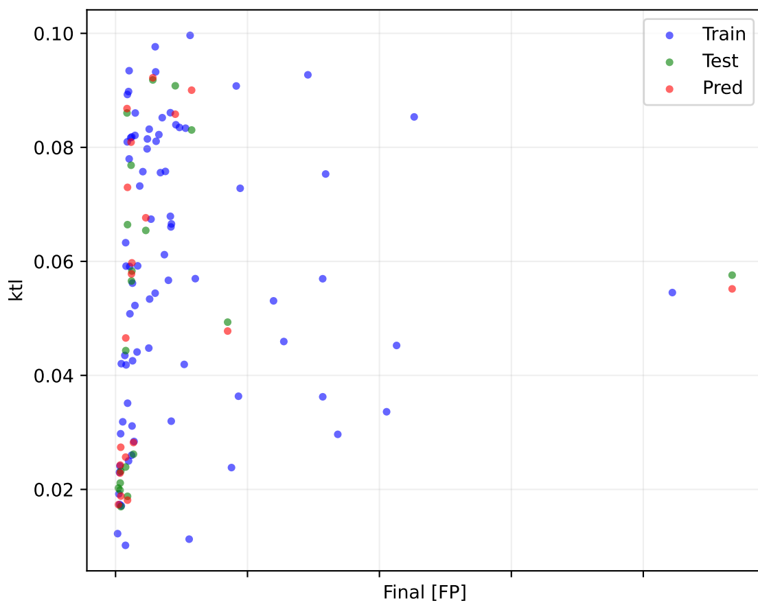
PILSTM Epoch 15000 lambda physics 0.0000
