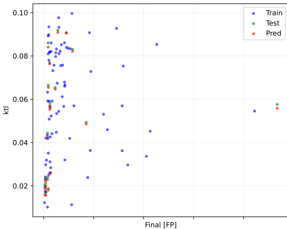
PILSTM Epoch 15000 lambda physics 0.0050
