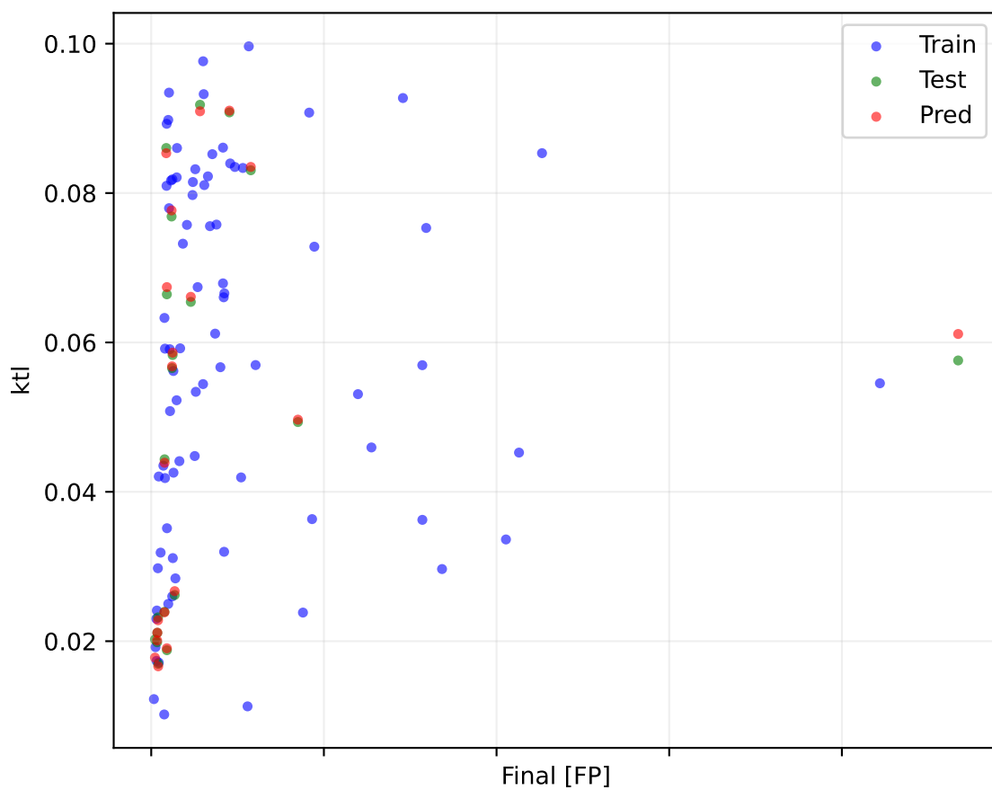
PILSTM Epoch 16000 lambda physics 0.0050
