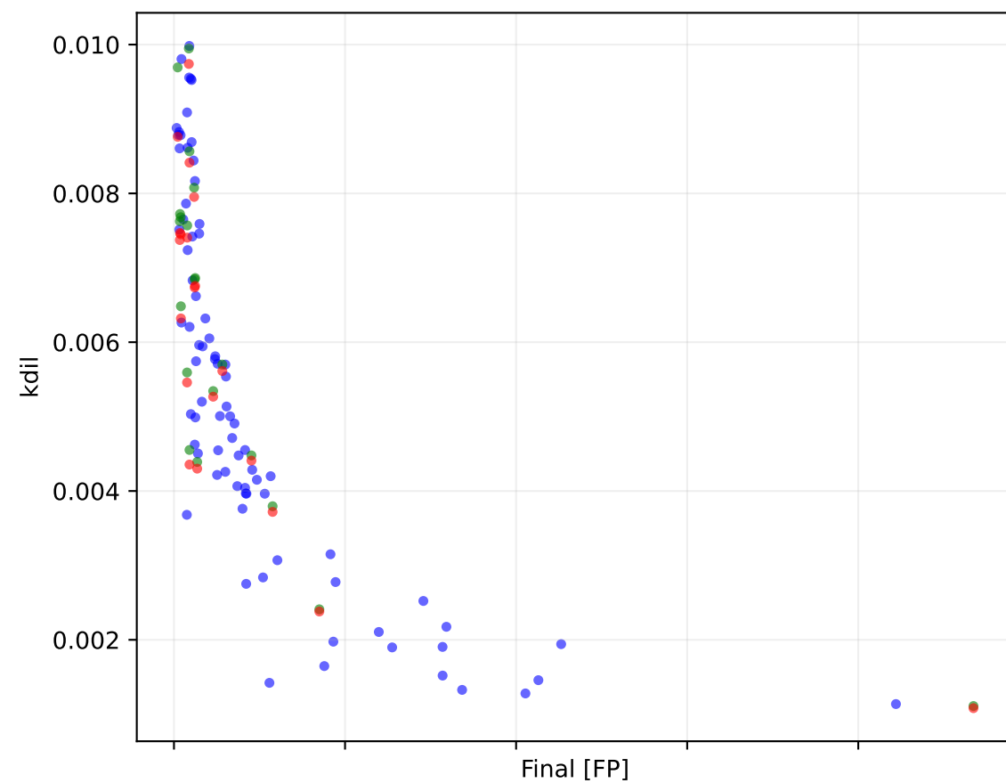
PILSTM Epoch 17000 lambda physics 0.0050
