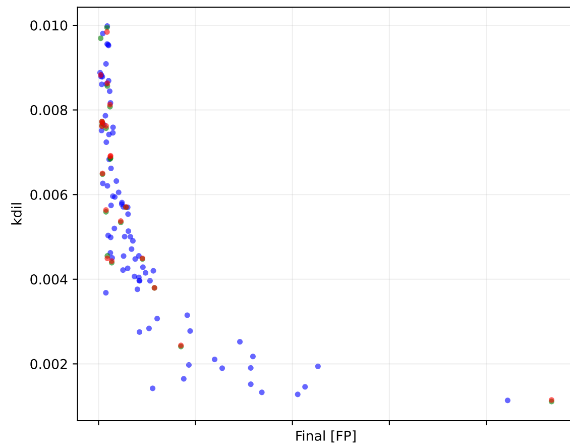
PILSTM Epoch 18000 lambda physics 0.0050
