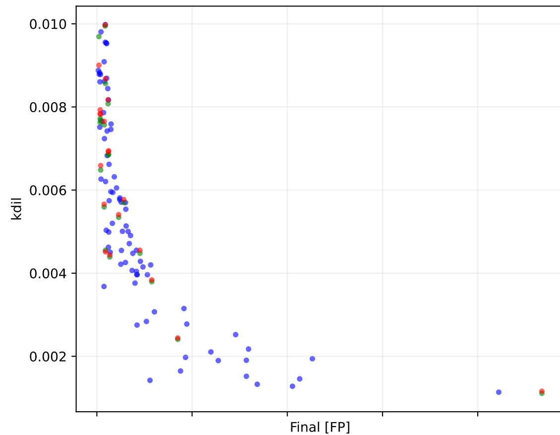
PILSTM Epoch 19000 lambda physics 0.0050
