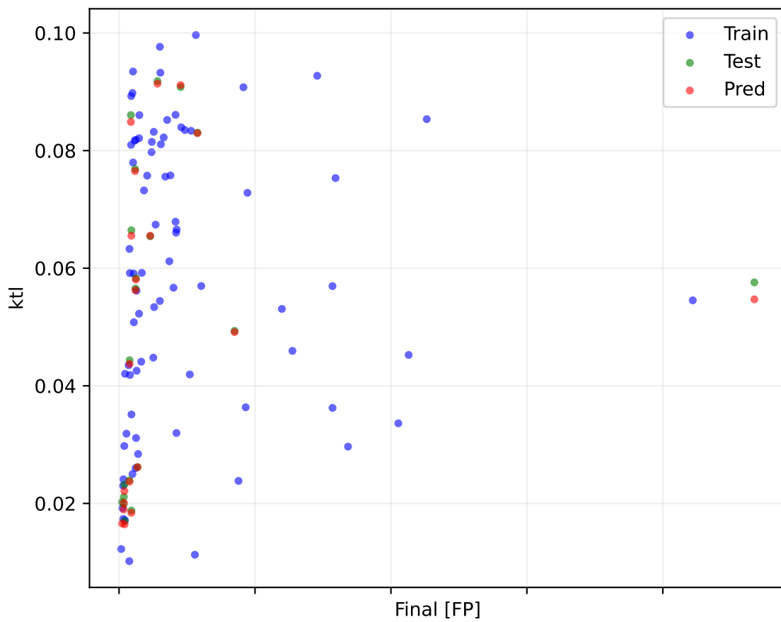
PILSTM Epoch 21000 lambda physics 0.0050
